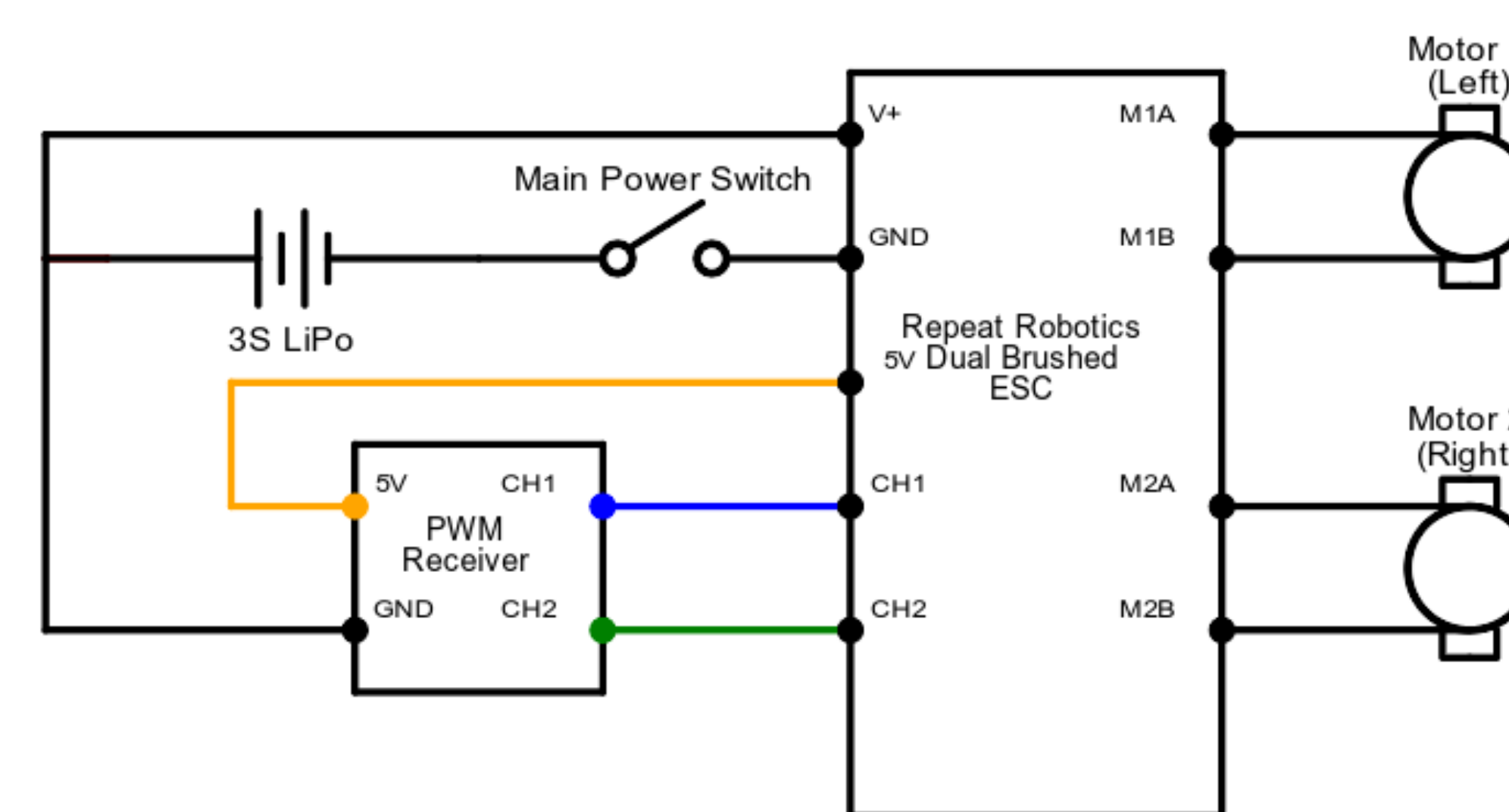
Figure 4: Electronics Diagram
